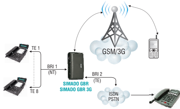
SIMADO GBR/SIMADO GBR 3G Stand-Alone Application
