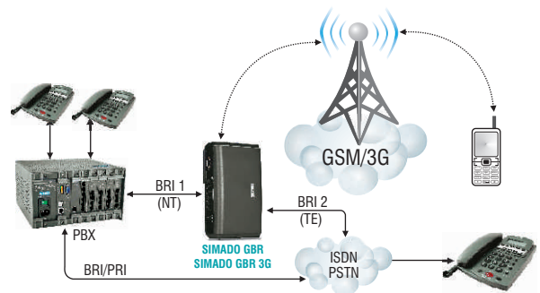
SIMADO GBR/SIMADO GBR 3G (NT) with PBX (TE) Application
